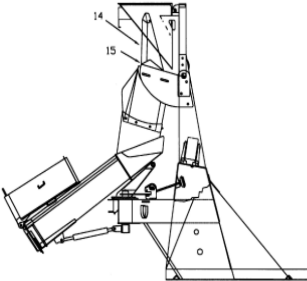
SMITH STANDARD MIXER FRONT & REAR PEDESTAL MODEL - LOW PROFILE
