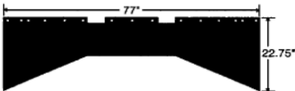
CB 1007G OSHKOSH HOPPER BIB OEM # 3HD524
