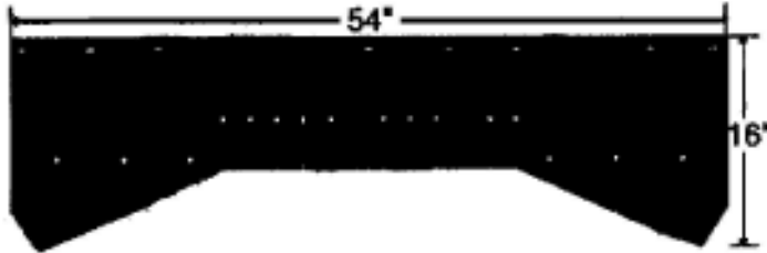
CB 1000 MTM HOPPER BIB 11 HOLE OEM # 120.115236A
